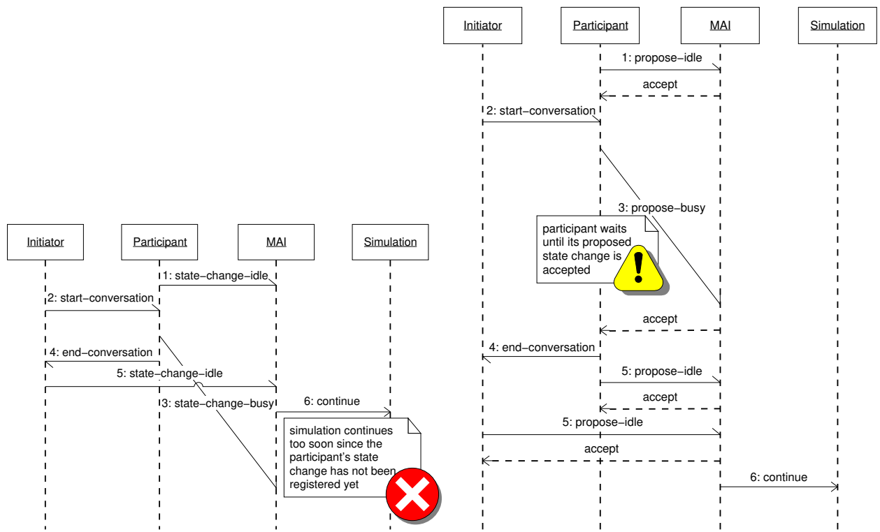
(a) State changes are not confirmed: Unsuccessful synchronization
