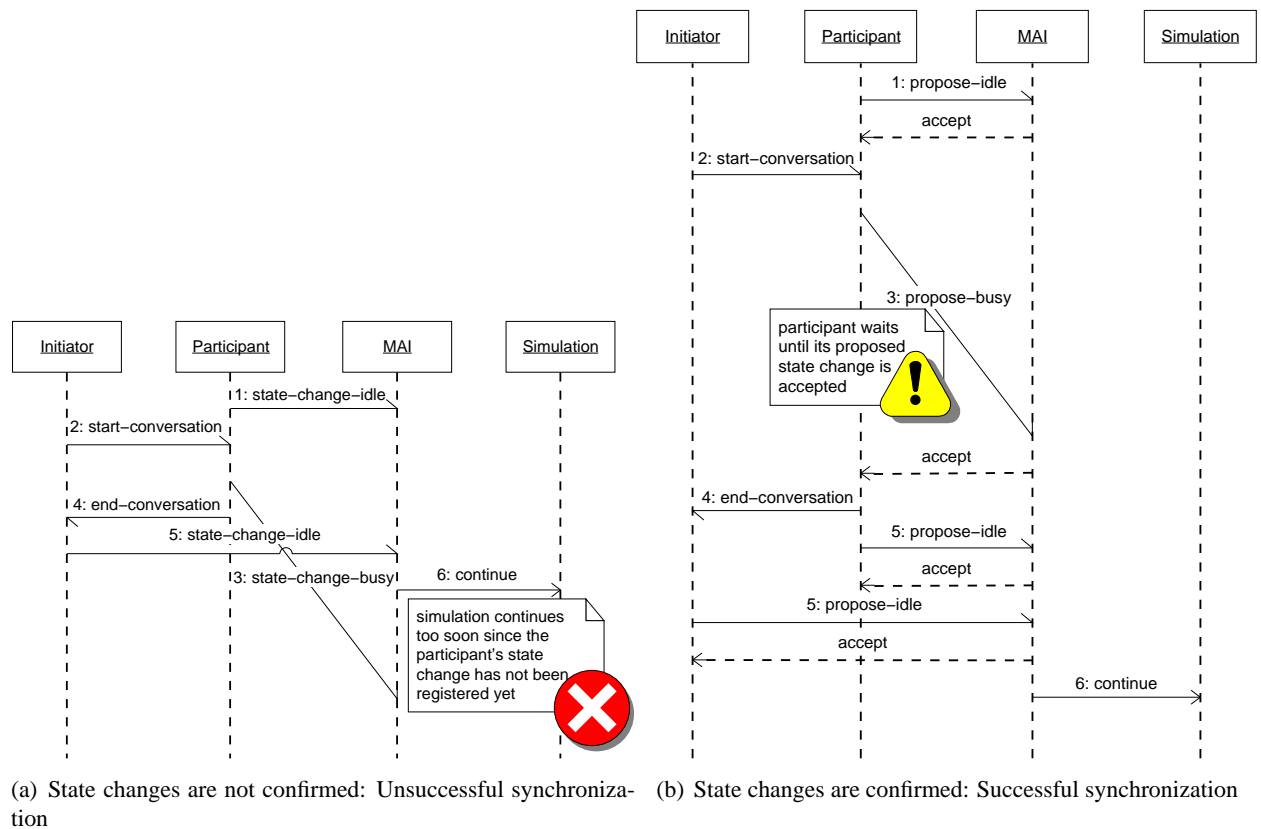
FIGURE 6 Synchronization sequences
