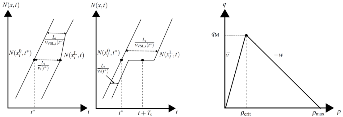
FIGURE 2: (a) Increase in the value of VSL, (b) Decrease in the value of VSL, (c) Triangular Fundamental Diagram.
