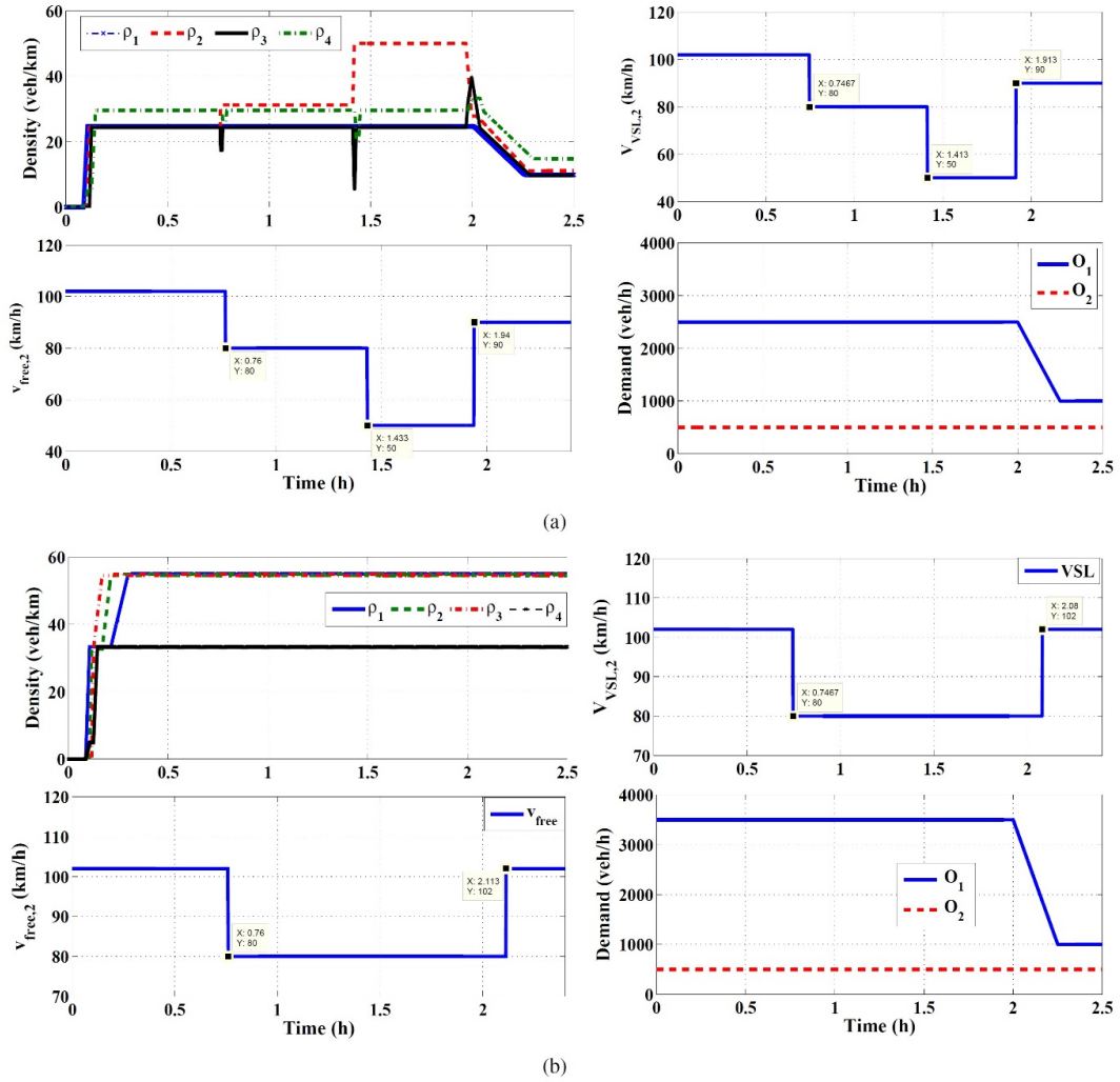
FIGURE 4:(a) Simulation results for (a) uncongested and (b) fully congested conditions.
