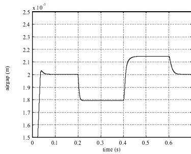
Figure 7: The air gap variation with nonlinear PD control and no noise on the sensor
