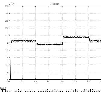
Figure 8: The air gap variation with sliding mode control and noise on the sensor
