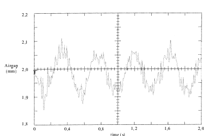
Figure 12: The variation of the air gap with linear PD control with the oscillating load variation
