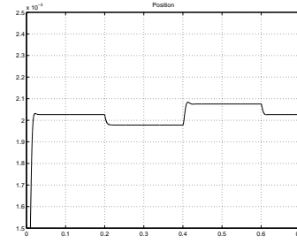
Figure 9: The air gap variation with sliding mode control and no noise on the sensor
