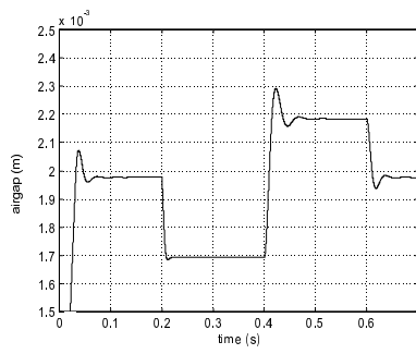
Figure 5: The air gap variation with linear PD control and no noise on the sensor
