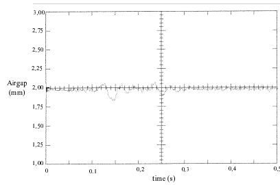
Figure 10: The variation of the air gap with linear PD control with mass of 0.1 kg falling from a height of 0.01 m
