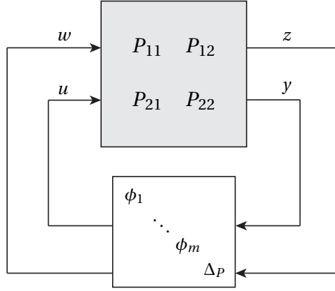
Figure 5.3: Closed-loop system including performance \Delta_P(s)
