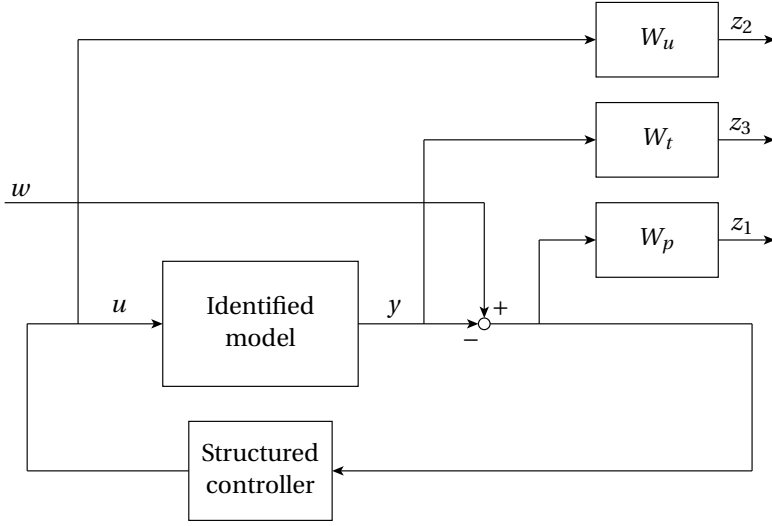
Figure 2.7: Mixed-sensitivity problem for structured LIP design.
