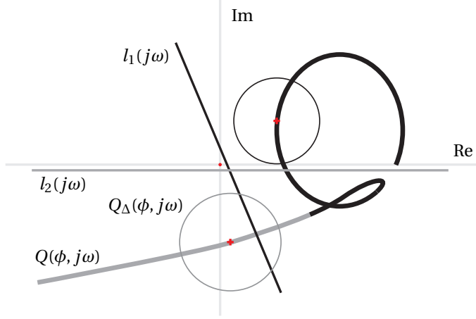
Figure 5.4: Nyquist diagram for Q(\phi, j\omega) (stability) and Q_\Delta(\phi, j\omega) (performance). The colors indicate which of the constraints l_1(j\omega) and l_2(j\omega) hold for which part of the Nyquist plots.
