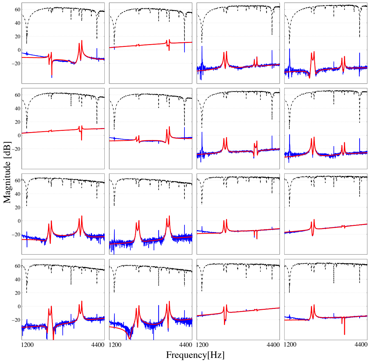
Fig. 1. Results with the AMB spindle system: amplitude plot of the FRF data G(\omega_k) (blue), the Schur weighting W_s(\omega_k) (black dash-dotted) and the estimated model P(\xi(\omega_k), \hat{\theta}) (red).
