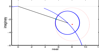
Fig. 2. Embedding an additive uncertainty (solid) with a v-gap uncertainty (dashed-dotted). The point in line with the nominal model G_x ('x') will cause the largest chordal distance.
