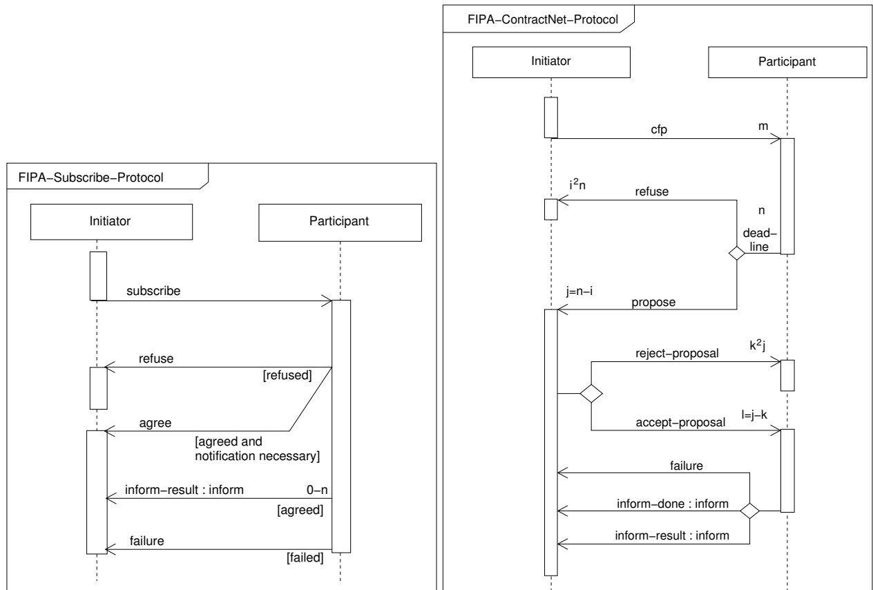
(a) FIPA subscription interaction protocol
