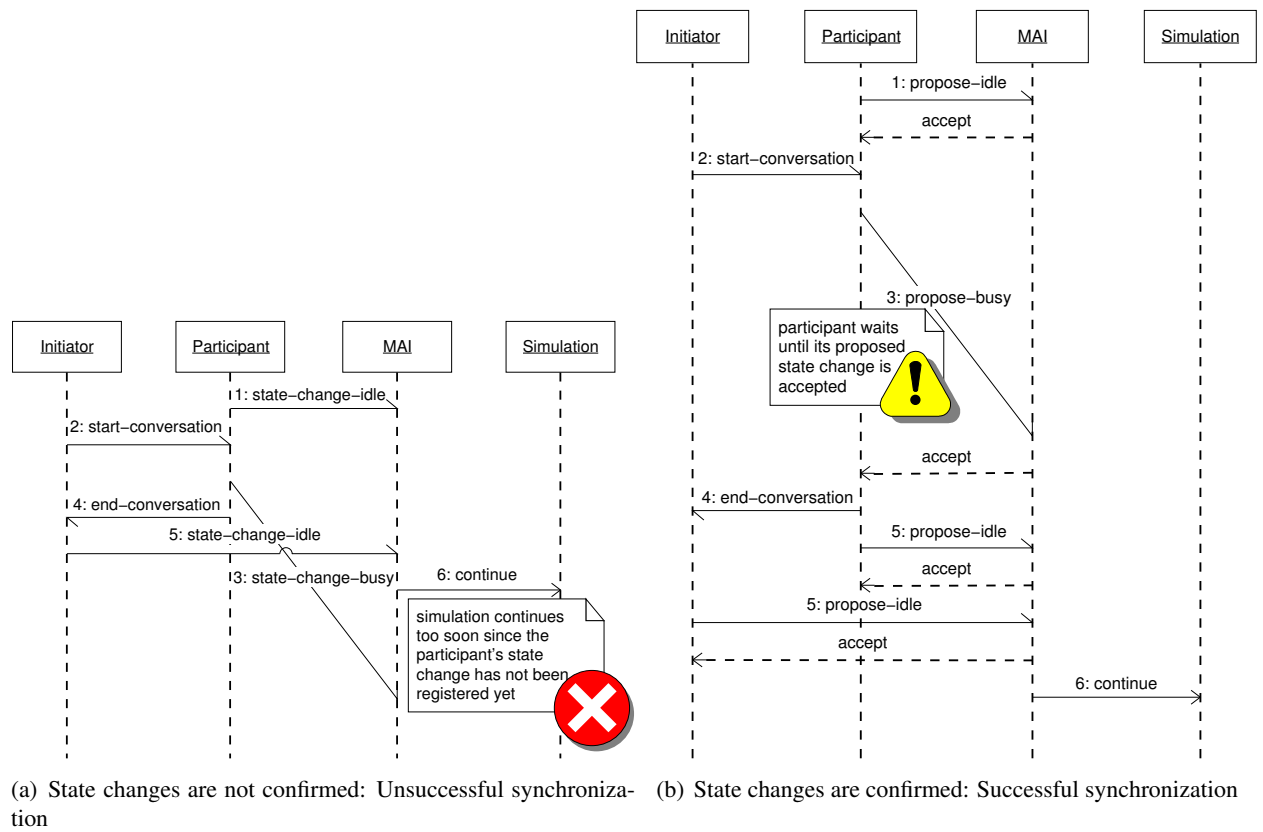
FIGURE 6 Synchronization sequences
