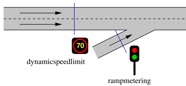
(a) The physical lay-out of the network. If the flows of the main-stream and on-ramp are too high, a traffic jam (bottleneck) will be created on the freeway at the on-ramp.
