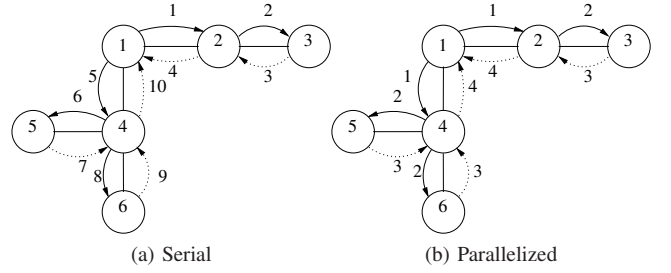
Fig. 1: Example of the order in which tokens can go. Solid arrows indicate computation tokens; dotted arrows indicate subgroup optimality information. The edges are labeled with the step within the iteration at which the information is sent.
