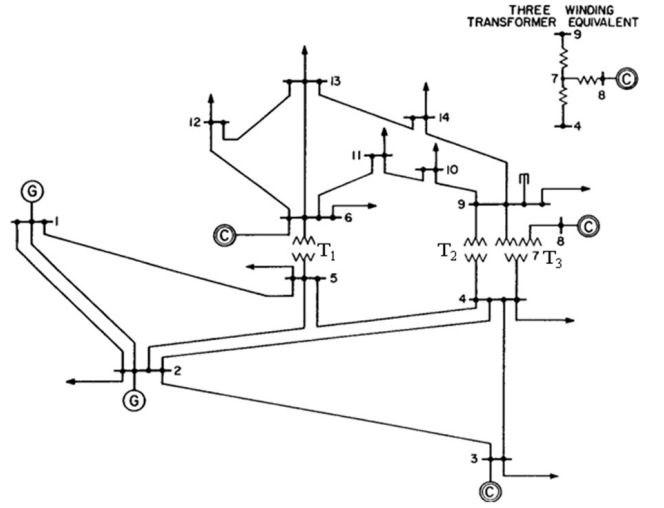
Fig. 1. IEEE 14 bus network which consists of 3 transformers [7].
