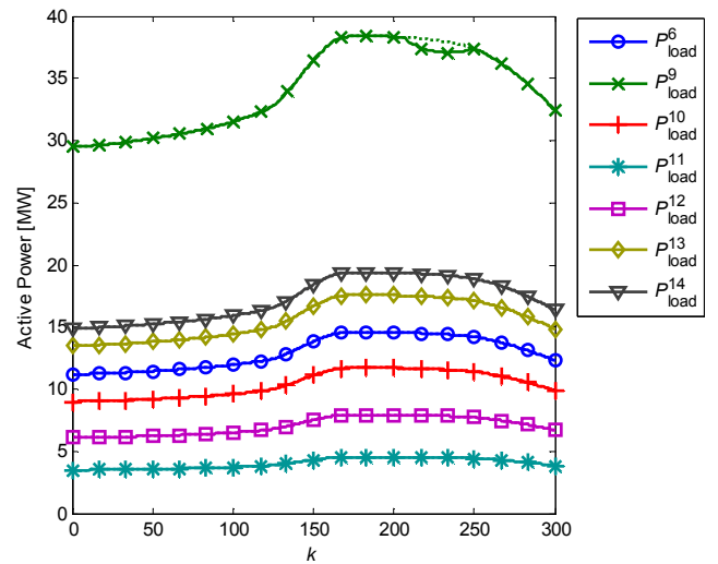
Fig. 2. Demand of the real power (dotted lines) and Actual real power delivered (solid lines) at buses of the distribution system.
