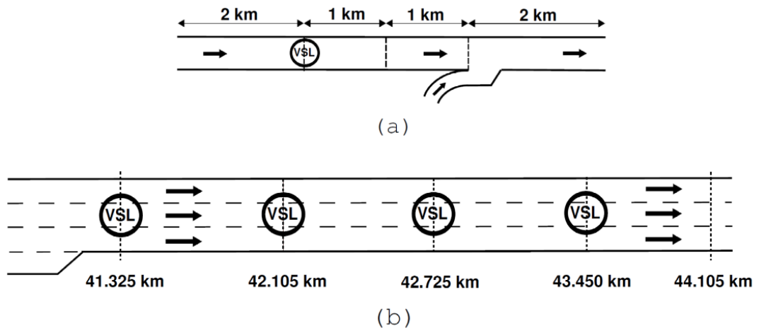
FIGURE 3: (a) Set-up of the case study, (b) Schematic VSL positions and links of the A12 freeway in The Netherlands.
