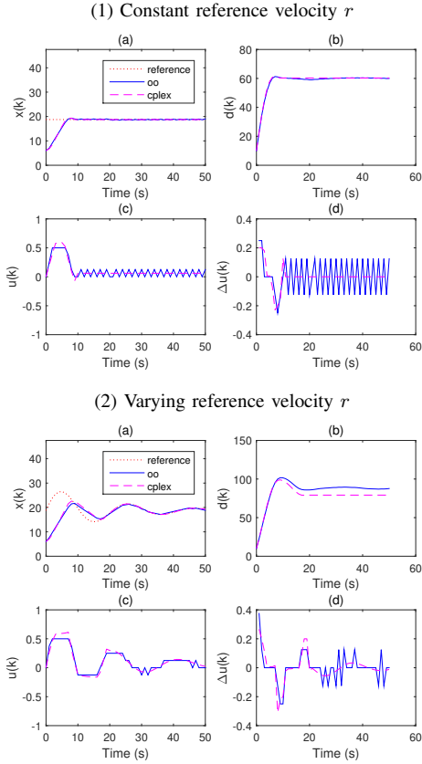
Fig. 2. Simulation results of cplex and optimistic optimization ( \circ\circ ) for constant and varying reference velocities ( t_{\max} = 10 for \circ\circ ): (a) Velocity of the follower vehicle; (b) Distance between two vehicles; (c) Control input; (d) Throttle/Brake variation
