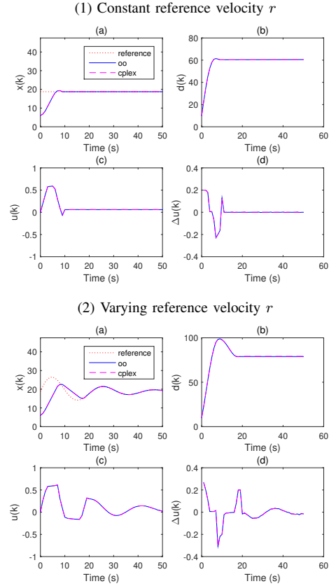
Fig. 3. Simulation results of cplex and optimistic optimization ( \circ\circ ) for constant and varying reference velocities ( t_{\max} = 1000 for \circ\circ ): (a) Velocity of the follower vehicle; (b) Distance between two vehicles; (c) Control input; (d) Throttle/Brake variation
