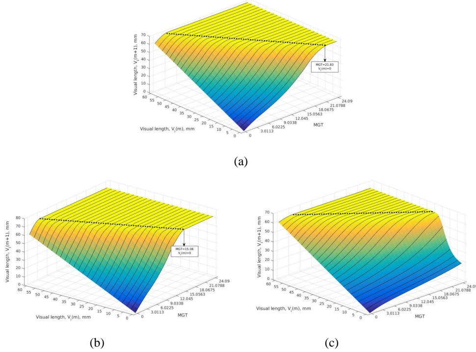
Fig. 5. Growth of squat visual length over MGT for the following model-based growth scenarios: (a) average, (b) fast, (c) slow, the dotted line depicts an upper bound of squat visual length.
