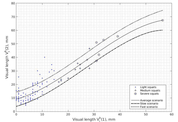
Fig. 4. Estimation of the visual length of the squats for m = 1 , and based on real data
