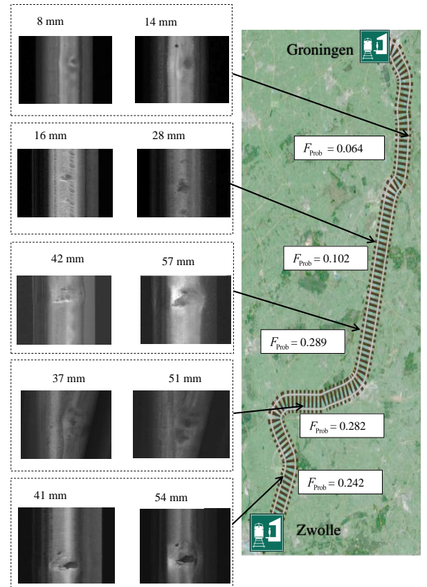
Fig. 10. A sample of failure risk estimates for 5 squats over the track
