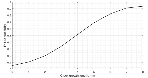
Fig. 9. Probability of rail failure based on the growth of crack length
