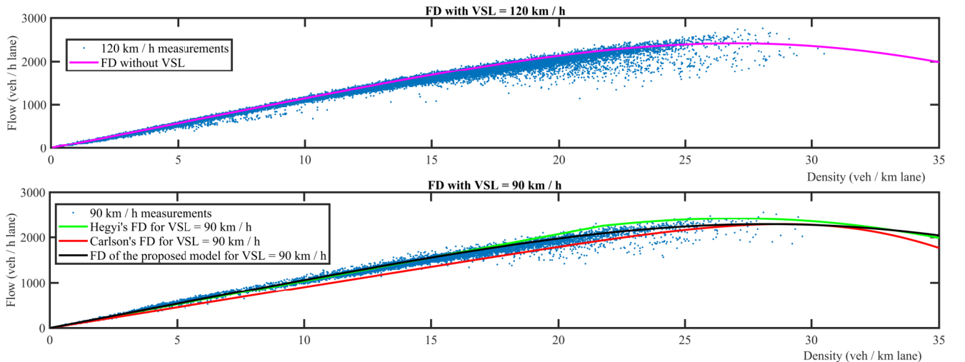
Fig. 5. Estimated FDs with v_{f,i} = 115 km/h, \rho_{c,i} = 27 veh/(km lane), a_i = 4 , V_{c,i}(k) = 90 km/h, \alpha_i = 0.15 (for Hegyi's model), A_i = 0.4245 and E_i = 5.5 (for Carlson's model), and \alpha_i = 0.18 , A_i = 0.388 and E_i = 0.4 (for the proposed model).
