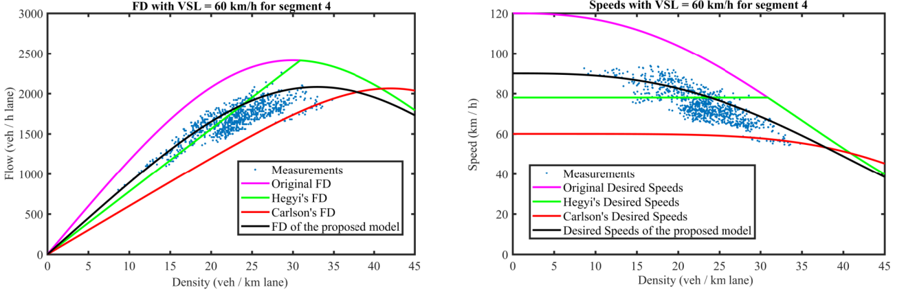
Fig. 6. FD diagrams and Desired Speeds for Link 4 with v_{f,i} = 120 km/h, \rho_{c,i} = 30 veh/(km lane), a_i = 2.5 , \alpha_i = 0.3 (for Hegyi's model), E_i = 3 , A_i = 0.8 (for Carlson's model), \alpha_i = 0.5 , E_i = 1.5 , and A_i = 0.4 (for the proposed model)
