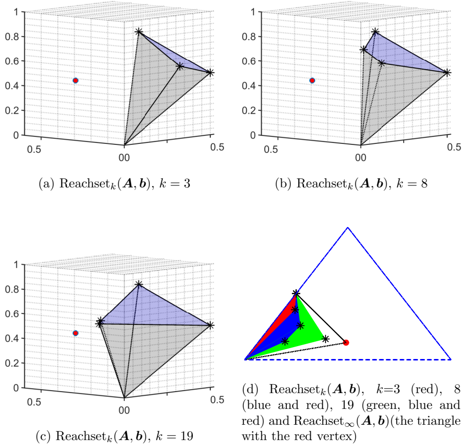
Fig. 2: a,b,c: The growth of the reachability cone \text{Reachset}_k(\mathbf{A}, \mathbf{b}) of Example 4.7 for different values of k , where generators of the cone are marked by asterisks, and the Frobenius eigenvector is marked by a red dot. d: The growth of the reachable cone mapped on the 3-dimensional simplex S = \{\mathbf{x} \in \mathbb{R}_+^3 \mid \mathbf{1}^T \mathbf{x} = 1\} .
