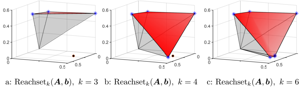
Fig. 4: Example 5.4: growth of the reachability cone mapped on the 3-dimensional simplex S = \{\mathbf{x} \in \mathbb{R}_+^3 \mid \mathbb{1}^\top \mathbf{x} = 1\} ; the generators of the cone and the Frobenius eigenvector are, respectively, marked by asterisks and a dot.
