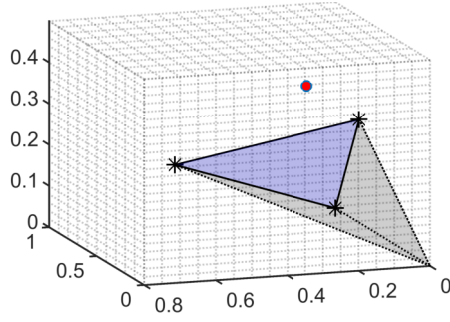
(a) \text{Reachset}_k(\mathbf{A}, \mathbf{b}) , k = 3
