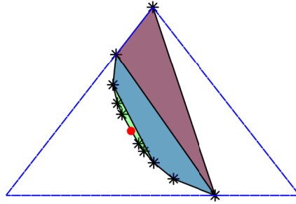
(d) \text{Reachset}_k(\mathbf{A}, \mathbf{b}) , k = 3 (red region), k = 6 (red and blue regions), k = 10 (red, blue and green regions). \text{Reachset}_\infty(\mathbf{A}, \mathbf{b}) approaches a “round cone”.
