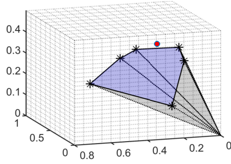
(b) \text{Reachset}_k(\mathbf{A}, \mathbf{b}) , k = 6
