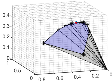
(c) \text{Reachset}_k(\mathbf{A}, \mathbf{b}) , k = 10
