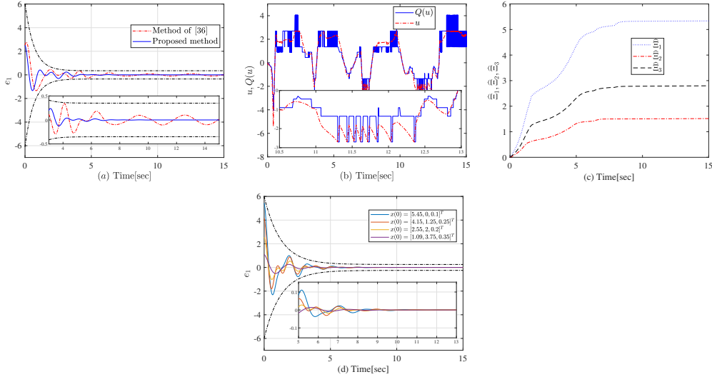
Fig. 2: Practical Example: (a) Evolution of tracking error e_1 under two schemes; (b) Evolution of the actual control signal u and the quantized control signal Q(u) ; (c) Evolution of adaptation parameters \hat{\Xi}_1 , \hat{\Xi}_2 , and \hat{\Xi}_3 ; (d) Evolution of tracking error e_1 under four different sets of initial conditions.
