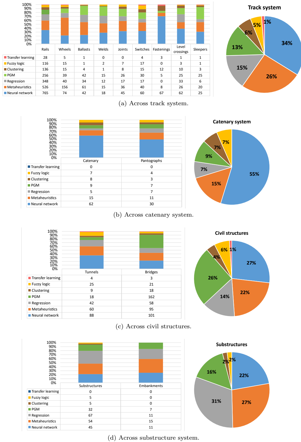
Figure 6. Distribution of the selected AI methodologies across the four groups of railway infrastructures. NB: one research paper can include multiple AI methodologies.
