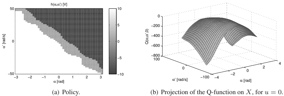
Figure 3.4: Results of LSPI with exact policy improvements on the servo-system.
