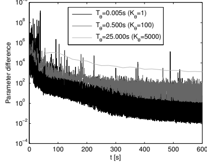
Figure 5.6: The evolution of parameter differences over time. Note that the parameter update frequencies are different between the three experiments. Parameter differences are computed with \|\theta_\ell - \theta_{\ell-1}\|_2 .
