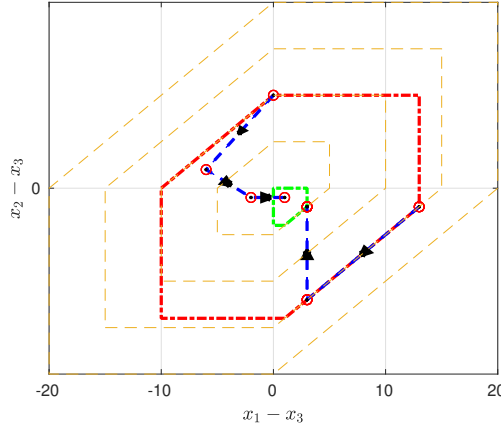
Figure 4.2: Max-plus C-set \mathcal{K} as defined in (4.8) (in green dash-dotted line -\cdot- ) and its level-set \widetilde{\mathcal{K}}_\mu , for \mu = 10 , (in red dash-dotted line -\cdot- ) projected on the hyperplane \{x \in \mathbb{R}^3 \mid x_3 = 0\} . Sample trajectories (in blue dashed line --- ) of the SMPL system defined by matrices in Example 4.3.1 are also shown. The level-sets of (symmetric) max-plus Hilbert balls centred at \mathbb{1}_n (in mustard --- ) represent practical bounds on the buffer-levels.
