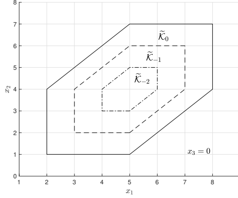
Figure 2.3: The max-plus cone generated by K in (2.24) as \text{span}_{\oplus}(\tilde{K}_{\mu}) are max-plus Hilbert balls for \mu \in \{0, -1, -2\} in \mathbb{R}^3 with a representative x_3 = 0 in the max-plus Hilbert projective space [196].
