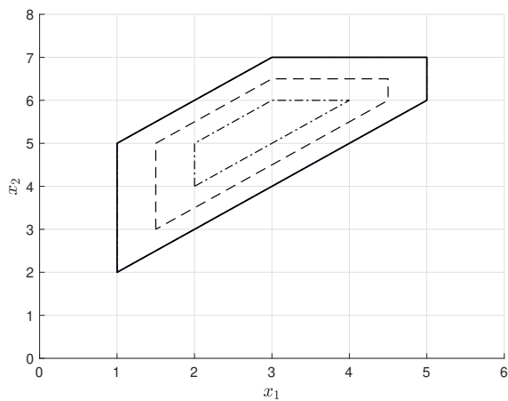
Figure 2.4: The max-plus cone generated by A and A^* in (2.25) as 2.4a \text{span}_{\oplus}(A) and 2.4b \text{span}_{\oplus}(\widetilde{A^*}_{\mu}) for \mu \in \{0, -0.5, -1\} in \mathbb{R}^3 with a representative x_3 = 0 in the max-plus Hilbert projective space \mathbb{R}^2 [196].
