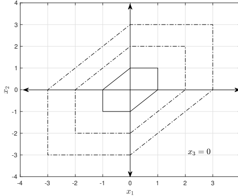
Figure 2.1: Concentric max-plus Hilbert balls \mathcal{B}_{\delta} of radii \delta \in \{1, 2, 3\} in \mathbb{R}^3 with a representative x_3 = 0 in the max-plus Hilbert projective space \mathbb{R}^2 .
