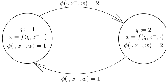
Figure 3.4: A max-plus-algebraic hybrid automaton visualisation of an SMPL system (3.1) with n_L = 2 modes. The function \phi(\cdot) encoding the switching mechanism appears in the definition of the mode invariants and as directed edge labels specifying the guard set for mode transition. The reset map is identity.
