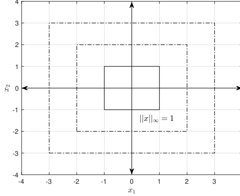
Figure 2.2: Concentric balls in the \ell^\infty norm of radii \delta \in \{1, 2, 3\} in \mathbb{R}^2 .
