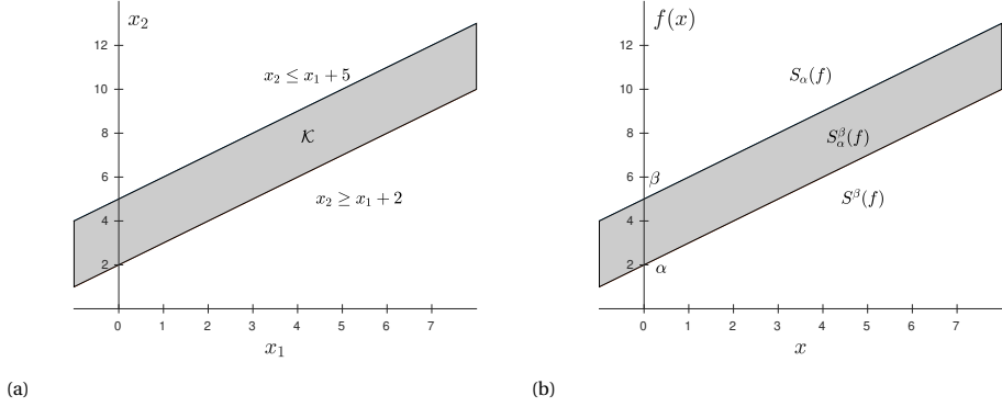
Figure 2.5: Max-plus cones: (a) Max-plus cone \mathcal{K} = \{(x_1, x_2)^\top \in \mathbb{R}_\epsilon^2 \mid x_1 + 2 \leq x_2 \leq x_1 + 5\} , and (b) Max-plus eigenspace S_\alpha^\beta(g) = S^\beta(g) \cap S_\alpha(g) for \alpha = 2 and \beta = 5 .
