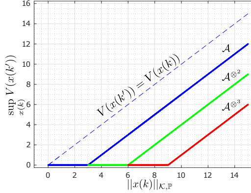
Figure 4.4: The worst-case convergence of trajectories of the open-loop switching max-plus linear system, in Example 4.3.3, to the max-plus C-set \mathcal{K} = \text{span}_{\oplus} K . The distance to the set is measured using the max-plus Lyapunov function V(x(k)) = x^*(k) \otimes K \otimes x(k) . The change in Lyapunov function, V(x(k)) - V(x(k')) , is minimised (as in Section 4.4.5) for k' = k + 1 , k' = k + 2 , and k' = k + 3 . This corresponds to the Lyapunov function decay for matrix semigroups \mathcal{A} , \mathcal{A}^{\otimes 2} , and \mathcal{A}^{\otimes 3} , respectively.
