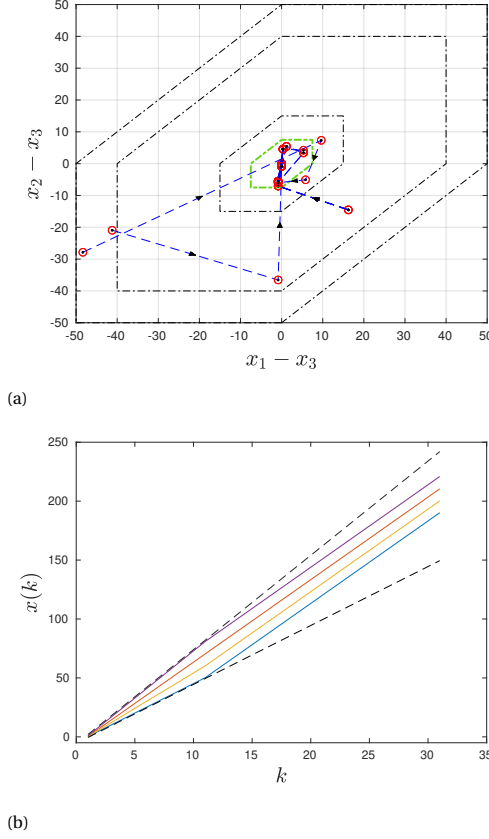
Figure 4.1: Notions of stability: (a) asymptotic max-plus bounded-buffer stability in a set \mathcal{K} (green dashed line - -) and (b) max-plus Lipschitz stability. The asymptotic stability for the first case is understood in the Lyapunov sense. In the latter case, the dashed (- -) lines represent the global bounds on the growth rates trajectories. Then asymptotic max-plus Lipschitz stability can be inferred from the eventual trajectories x(k) .
