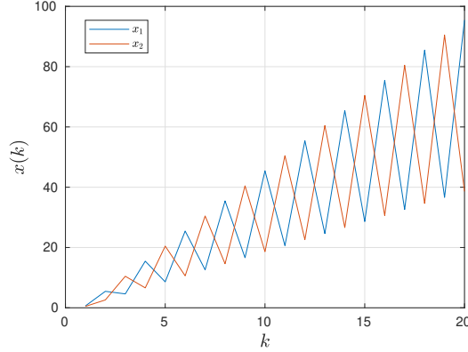
Figure 4.3: Trajectory of the open-loop switching max-plus linear system defined in Example 4.3.2 under periodic switching \sigma = 1, 2, 1, 2, 1, \dots . Note that \|x(k)\|_{\mathbb{P}} and \max_i (x_i(k) - x_i(k-1)) diverge along the event step k \in \mathbb{N} .
