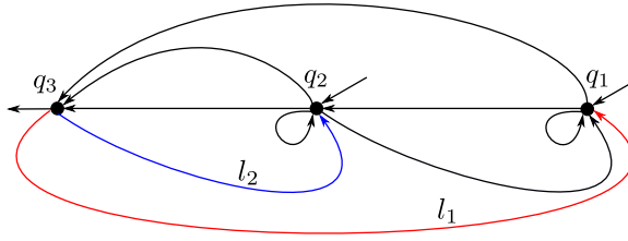
Figure 3.7: The one-step state transition graphs associated to the production network in Fig. 4.3. The finite automaton can be obtained by duplication of the nodes q_1 - q_3 for the two modes l_1 and l_2 . The black arcs are common to both the modes. The blue arc (—) belongs to mode l_2 and the red arcs (—) belong to mode l_1 . The input and output arrows symbolise the initial and final states of the finite automaton.
