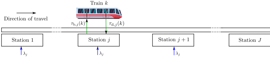
Figure 5.1: Unidirectional urban railway line with J stations and K trains. The boarding and disembarking times for each train k \in \underline{K} at any given station j \in \underline{J} are denoted as \tau_{b,j}(k) and \tau_{d,j}(k) , respectively. Passengers arrive at a constant rate \lambda_j per unit time at all the stations. The passengers alight the train at a constant rate b per unit time.
