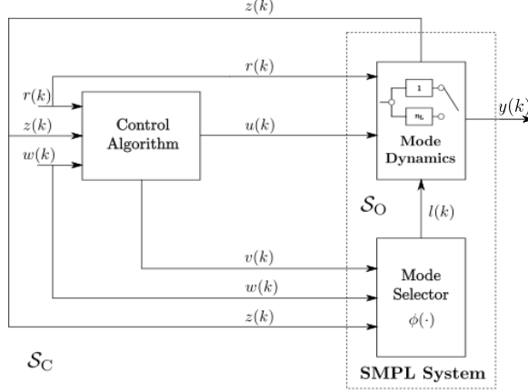
Figure 3.1: The SMPL system in closed loop \mathcal{S}_C with a controller, represented as a subclass of the class of discrete hybrid automata.
