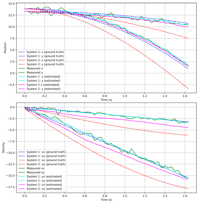
Figure 7.4: Comparison of estimated states for MHE with different dynamics constraints. The measured trajectories correspond to an object of Class 1.
