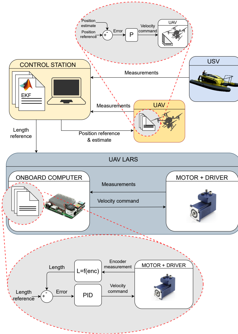
Figure 4.14: Tethered UAV control scheme overview.
