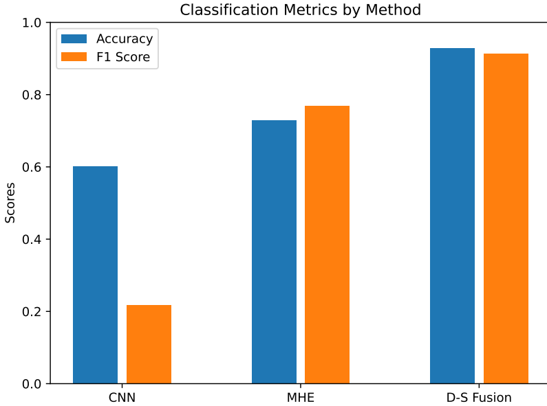
Figure 7.5: Performance comparison of each classifier and their D-S fusion.
