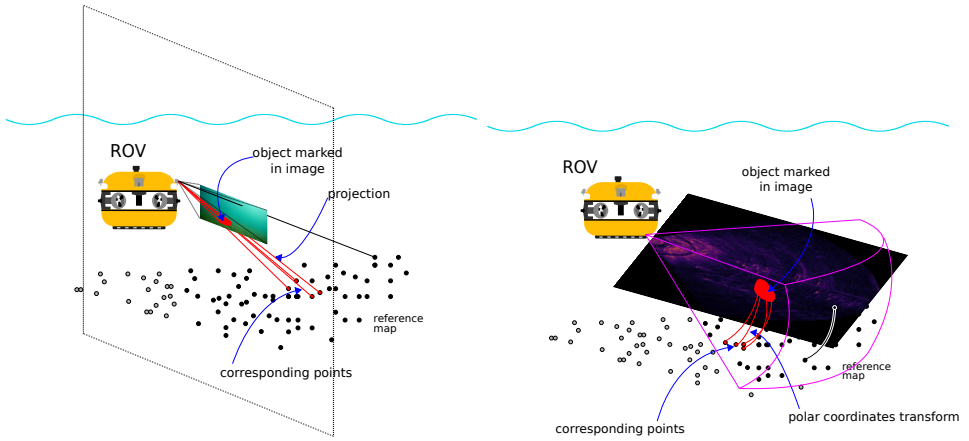
Figure 4.10: Left: Mapping from a marked camera image. The pre-selected points are shown in black, and the projection from the point cloud into the image by lines. The red object in the camera image corresponds via the red lines to the object points in the point cloud, also shown in red. Right: Mapping from a marked sonar image. The symbolism is similar to the camera mapping. One difference is that here the black points are pre-selected using the more complicated shape of the sonar field of view, shown in a red outline.
