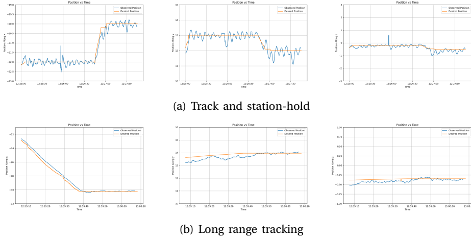
Figure 4.24: Tracking performance of the Collection ROV from Hamburg port demonstrations.
