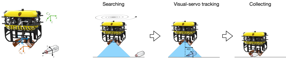
Figure 4.12: (Left) Depiction of the inertial frame ( C_J ), the vehicle-frame ( C_V ), the body-fixed frames of the camera ( C_c ), the gripper ( C_g ), and the frame of the object of interest ( C_o ) (Right) Grasping phases: If no object is directly found at the map coordinates, a spiral search pattern is followed until a litter object is detected in the gripper-camera image. With the object in sight, visual-servo tracking centers the object in the gripper frame during the decent. Once the object is in reach it is collected for transportation to the basket.
