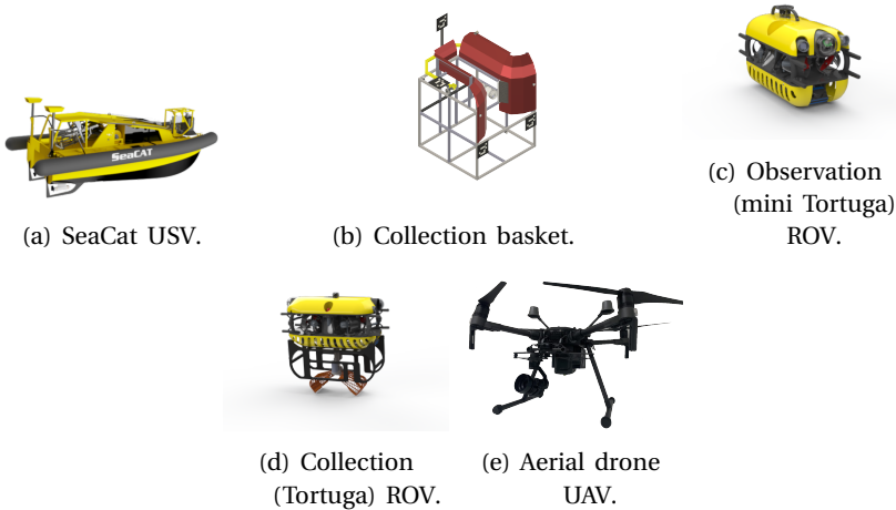
Figure 4.2: SeaClear system modules.
