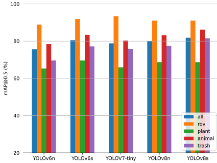
Figure 6.6: Performance of clear water environment specific models trained with several YOLO architectures, validated on all clear water datasets.
