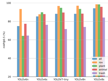
Figure 6.5: Performance of environment generalist models trained with several YOLO architectures, validated on the SeaClear dataset.
