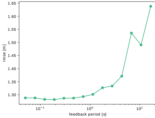
Figure 4.22: RMSE between pose estimate and SBL obtained for a range of UAV feedback period choices.
