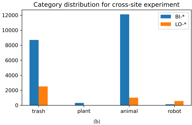
Figure 3.6: Category distributions for domains used in cross-camera and cross-site experiments.
