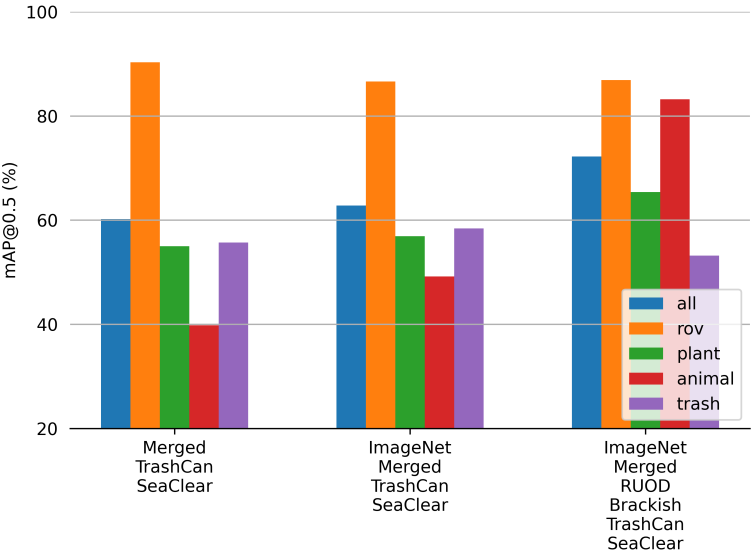
Figure 6.3: Effect of merged datasets on generalization performance.
