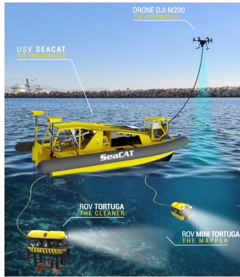
Figure 4.1: Overview of the SeaClear robotic platform
