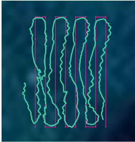
Figure 4.23: Planned waypoints (magenta disks) connected by lines, and actual trajectory (teal) of the ROV.
