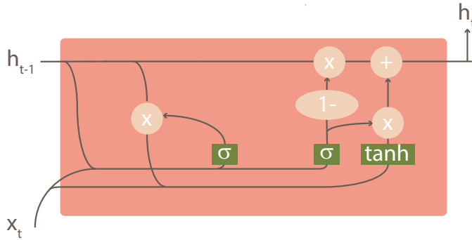
Figure 2.4: GRU structure, adapted from [305]
