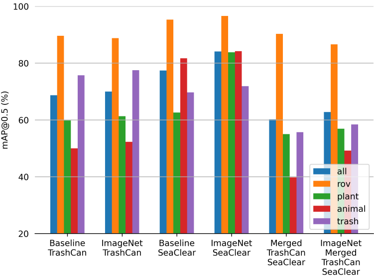
Figure 6.2: Effect of underwater specific pretraining with ImageNet.
