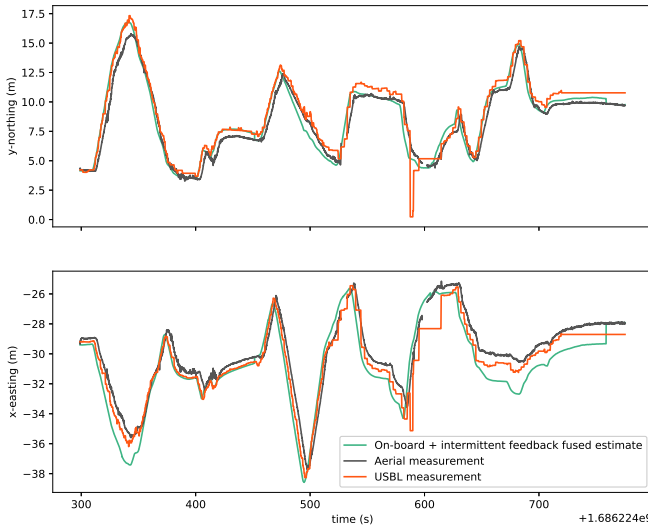
Figure 4.21: Pose estimation result: evolution over time of the planar positions X and Y . The horizontal axis depicts Unix epoch time in seconds.
