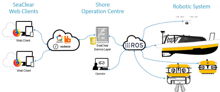
Figure 4.4: Overview of the SeaClear software architecture.
