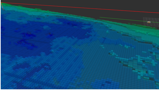
Figure 4.15: Red: The planner bounds. Green: A downsampled path planned by the RRT* algorithm in the simulated octomap created from real bathymetry data.
