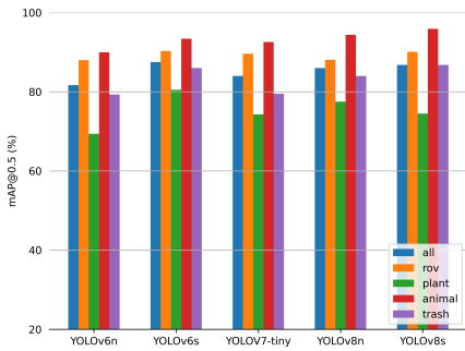
Figure 6.8: Performance of brackish water environment specific models trained with several YOLO architectures, validated on all brackish water datasets.
