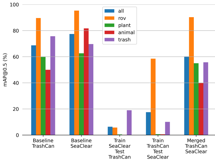
Figure 6.1: Baseline, cross-dataset & merged TrashCan and SeaClear dataset evaluation.
