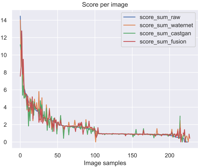
Figure 5.6: Classification score among methods.
