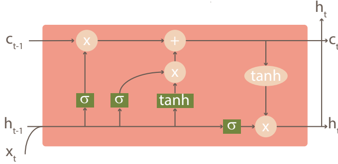
Figure 2.3: LSTM cell structure, adapted from [305].
