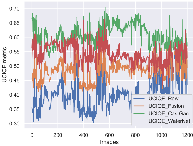
Figure 5.7: UCIQE metric per image for each method.
