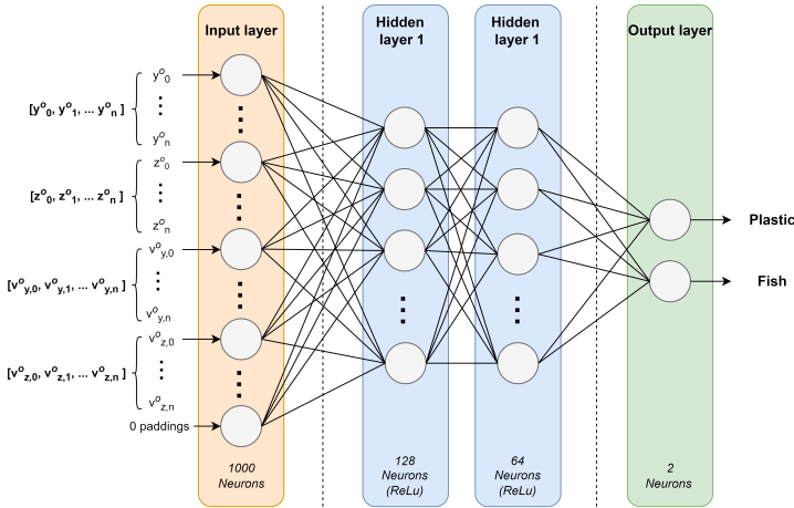
Figure 8.6: Architecture of the neural network used to classify the underwater moving objects
