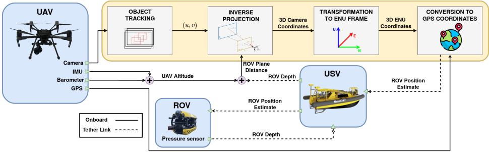
Figure 4.6: Scheme of the ROV position estimation from the UAV adapted from [53]. The ROV reports its own current depth, necessary to compute the ROV position estimate onboard the UAV. This estimate is then reported back to the ROV and used as an external input for the full ROV pose estimation algorithm.
