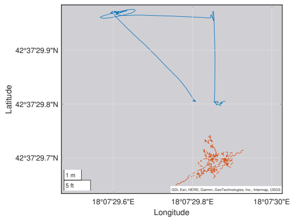
Figure 4.27: UAV GPS position (blue) and UAV LARS GPS position (red dashed) in the SeaClear Lokrum Demo.
