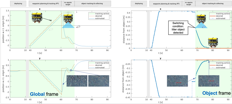
Figure 4.19: Simulation of the full automated collection sequence based on live object detection. The green shaded areas highlight the active tracking in global and object coordinate frame, respectively. Upper plots show the x -coordinate, lower plots the y -coordinate in the respective frame. Both plots show convergence of tracking in the object frame towards the center of the camera frame for picking up the object with the camera-aligned gripper.
