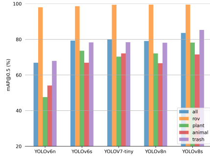
Figure 6.7: Performance of clear water environment specific models trained with several YOLO architectures, validated on the clear water portion of the SeaClear dataset.
