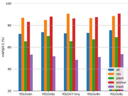
Figure 6.4: Performance of environment generalist models trained with several YOLO architectures, validated on all datasets.
