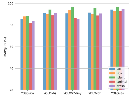
Figure 6.9: Performance of brackish water environment specific models trained with several YOLO architectures, validated on the brackish water portion of the SeaClear dataset.
