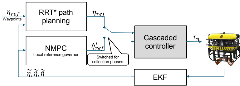
Figure 4.11: Control structure of the Collection ROV with switching reference inputs during path tracking and the collection sequence.
