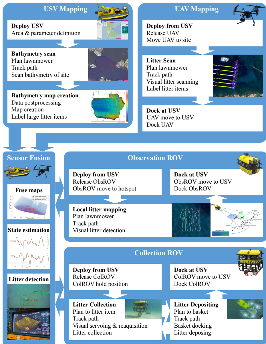
Figure 4.5: Overview of the SeaClear mode of operation.
