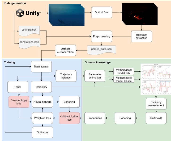
Figure 8.7: Overview of the proposed architecture for training the classifying neural network
