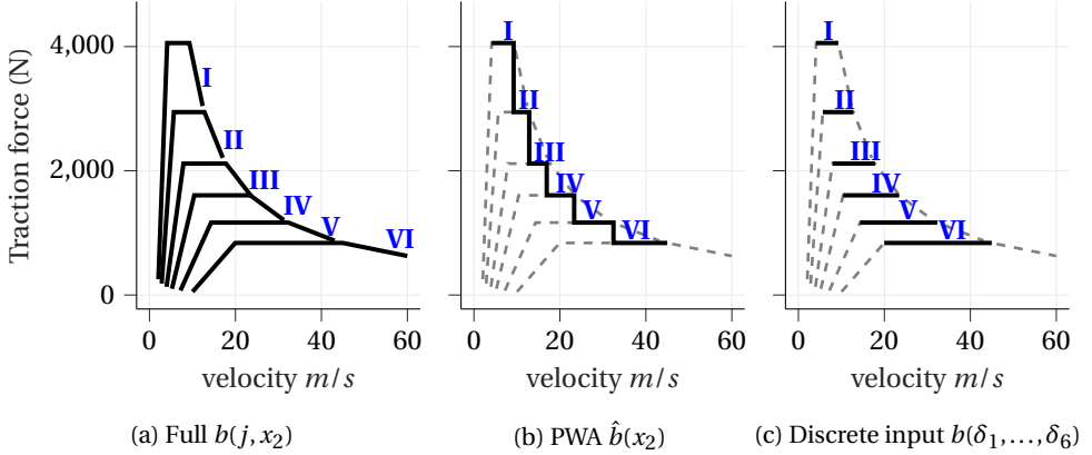
Figure 8.2.: Gear models.
