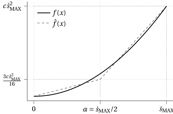
Figure 8.1.: PWA friction approximation. True quadratic function (solid), piecewise approximation (dashed).
