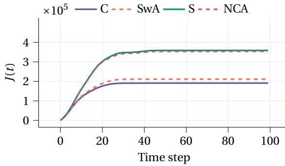
Figure 3.8.: Cumulative tracking cost for M = 10 .
