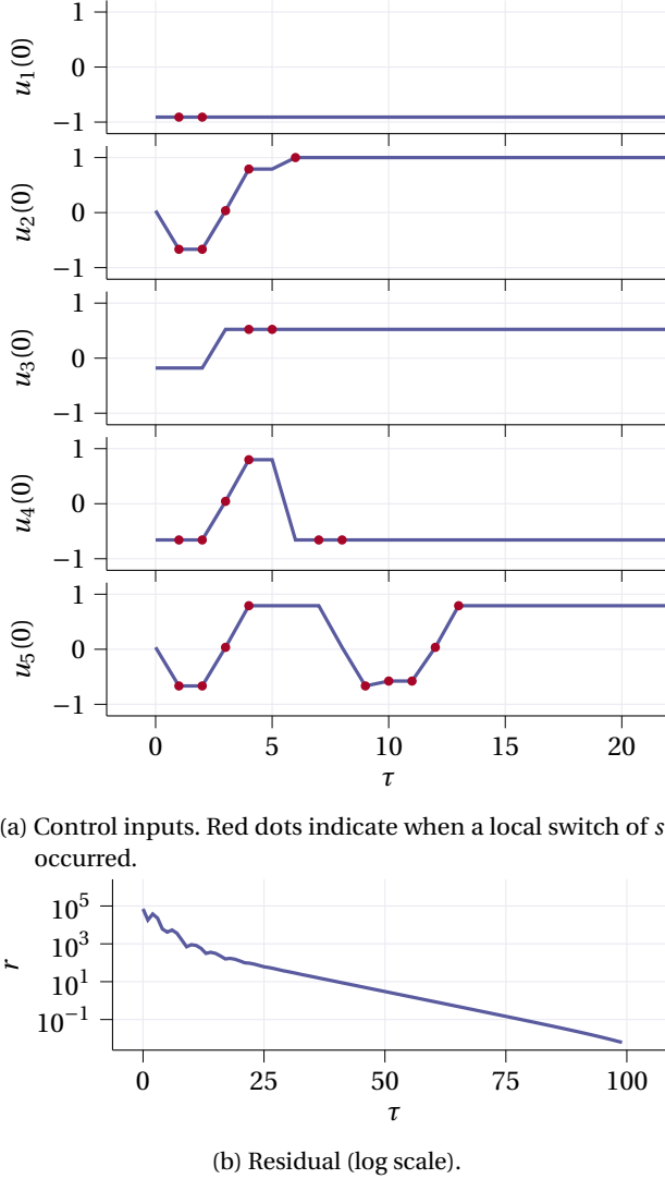
Figure 3.7.: Iterations of Algorithm 3.3.
