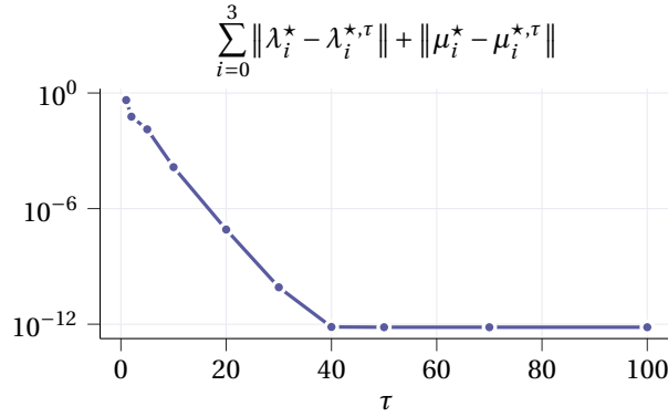
Figure 4.1.: Accuracy of the dual variables recovered by Proposition 4.2 as a function of the ADMM iteration index \tau
