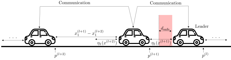
Figure 8.3.: Platoon control.
