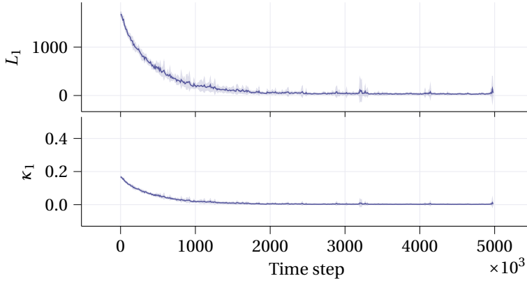
Figure 7.3.: Performance metrics over the training stage 1. The plots show mean (solid) and standard deviation (shaded) of the moving average of the metrics for a moving window of 10000 steps.
