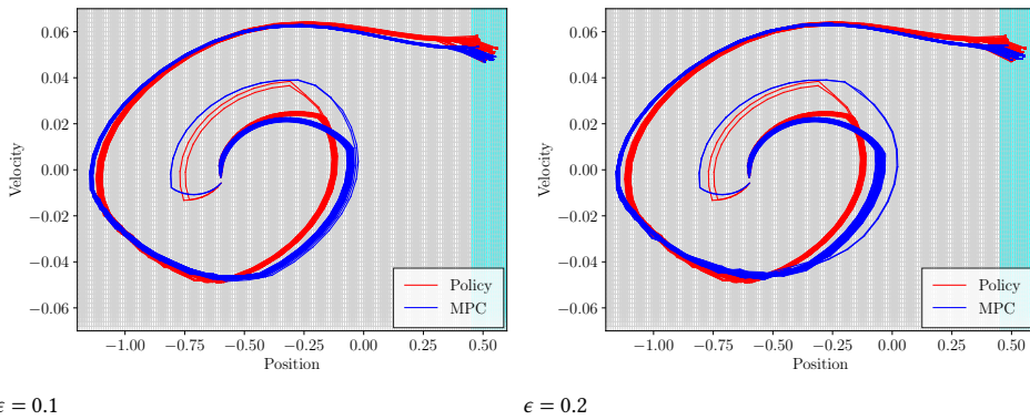
Figure 5.7: Mountain car simulations with different \epsilon for the baseline (policy; red) and our MPC controller (blue).
