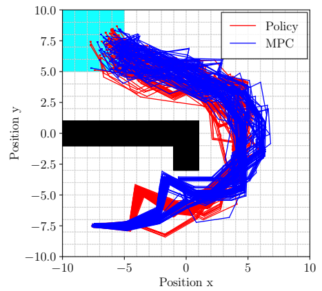
Figure 5.8: Dubins simulations with different \epsilon for the baseline without MPC (policy; red) and our MPC controller (blue).
