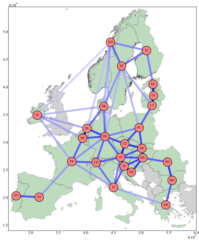
Figure 2.1: Electrical topology of the EEA-ENB. Each node represents an electrical area, coinciding with a single country, whereas each edge is a transmission line. The transparency of the edges represents the strength of interaction among the areas.
