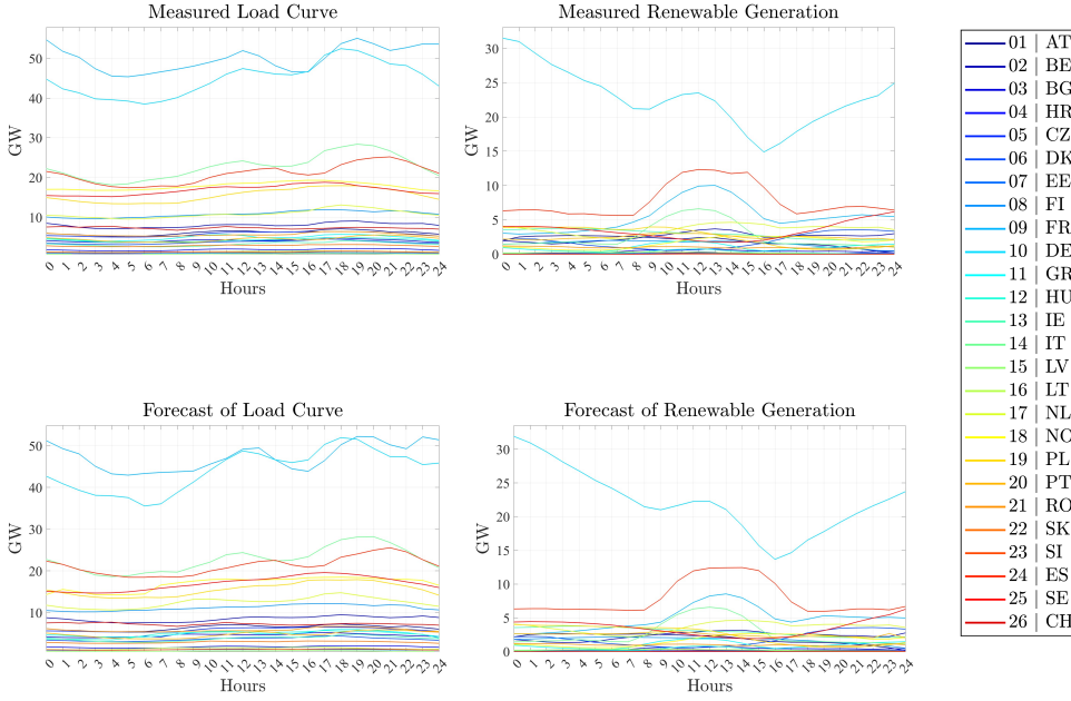
Figure 2.3: Measurements and forecasts of the load request and renewable generation of each electrical area.
