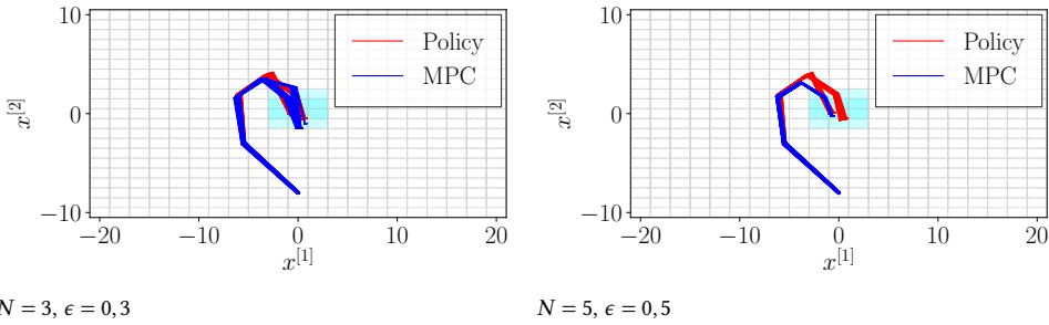
Figure 5.6: Simulated state trajectories for the double integrator, showing the baseline without MPC (policy) and the MPC.
