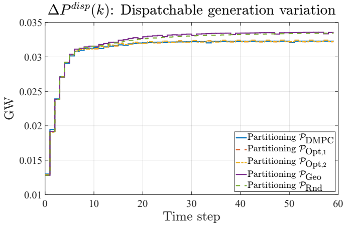
Figure A.4: Evolution of dispatchable generation.
