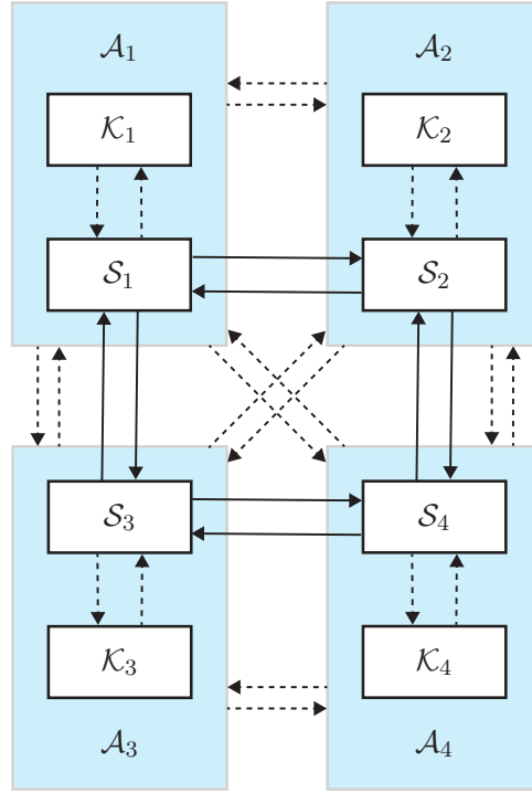
Figure 4.1: A network of control agents. Subsystems are indicated by S , local controllers by K , and control agents by A . The solid lines represent the interactions at the physical level, i.e. the dynamical couplings; instead, the dashed lines represent interactions at the information level.
