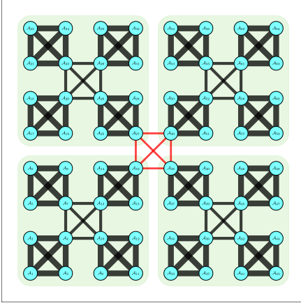
Partition \mathcal{P}_3
