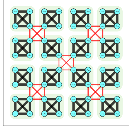
Partition \mathcal{P}_2
