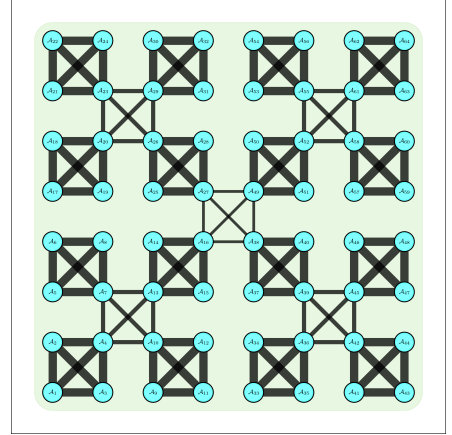
Partition \mathcal{P}_4
