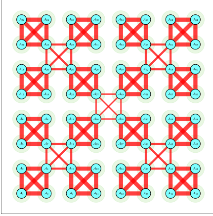
Partition \mathcal{P}_1
