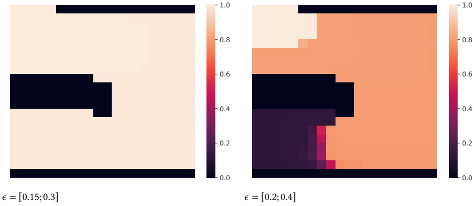
Figure 5.5: Heat maps of the lower bound of the satisfaction probability for the Dubins car.
